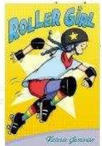
FORCES
