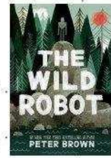
ELEMENTS
