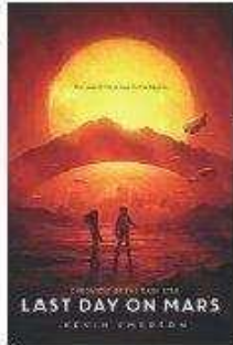
SPACE PHYSICS
