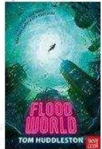
CLIMATE CHANGE
