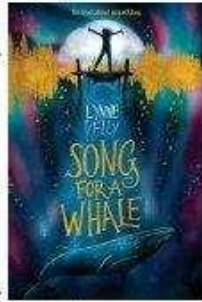
SOUND
