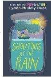
CLIMATE
