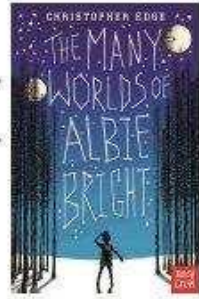
PHYSICS
