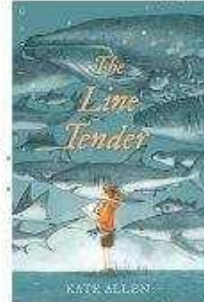
BIOLOGY
