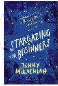
SPACE PHYSICS
