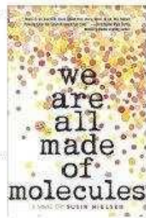
CHEMISTRY
