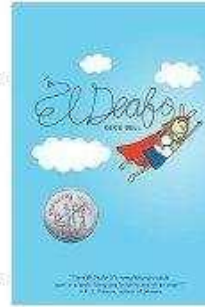
SOUND
