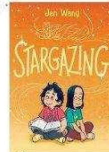
SPACE PHYSICS
