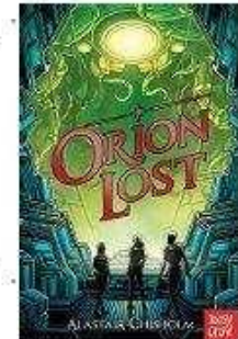
SPACE PHYSICS
